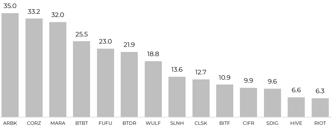
EV / Hashspread (1) (x)
