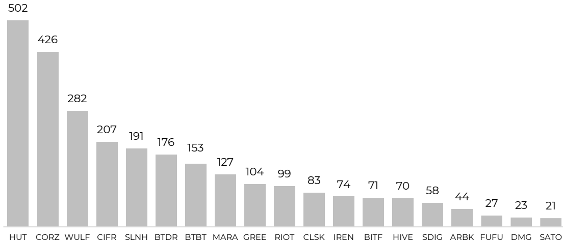
EV / Hashspread (1)
