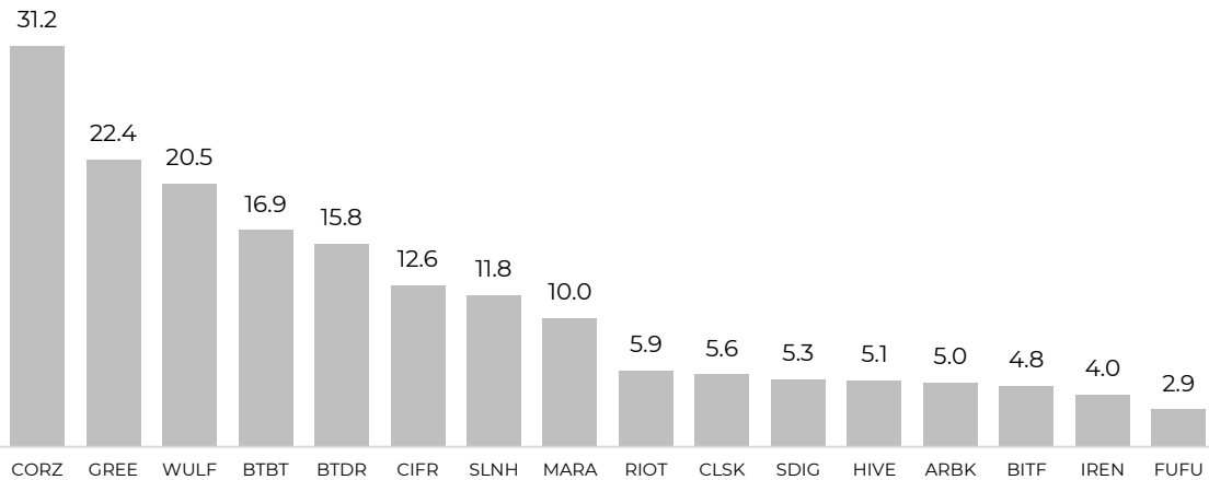
EV / Hashspread (1)
